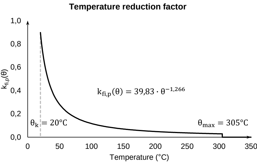
Figure C5: Reduction factor k_{fi,p}(\theta)
